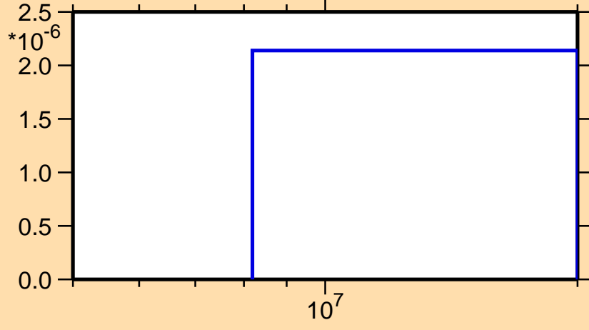
\sigma vs. E for ^{102}\text{Zr}(n,\alpha)
