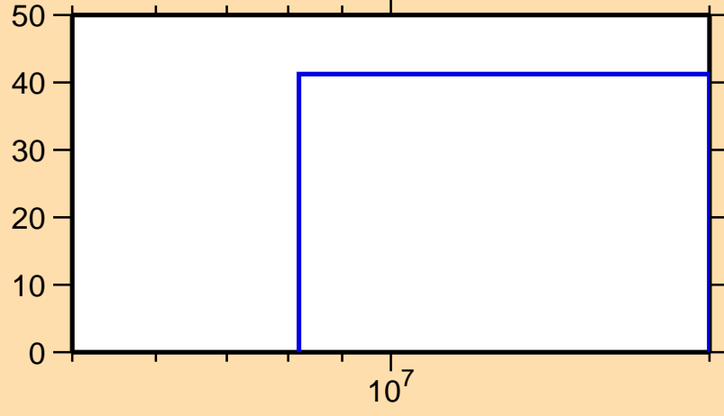
\Delta\sigma/\sigma vs. E for ^{102}\text{Zr}(n,n\text{cont.})
