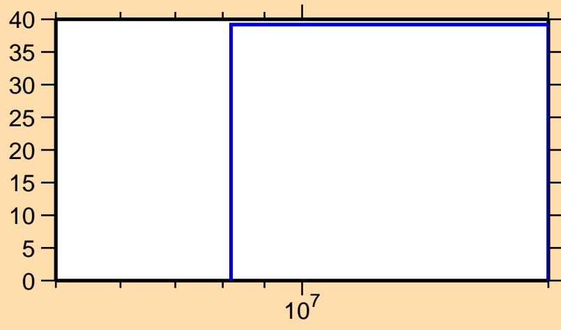
\Delta\sigma/\sigma vs. E for ^{102}\text{Zr}(n,p)
