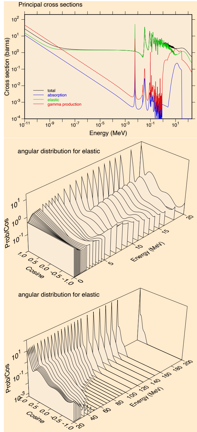
Fig. 1. \text{Al}^{27} Principal cross section and angular distribution.
