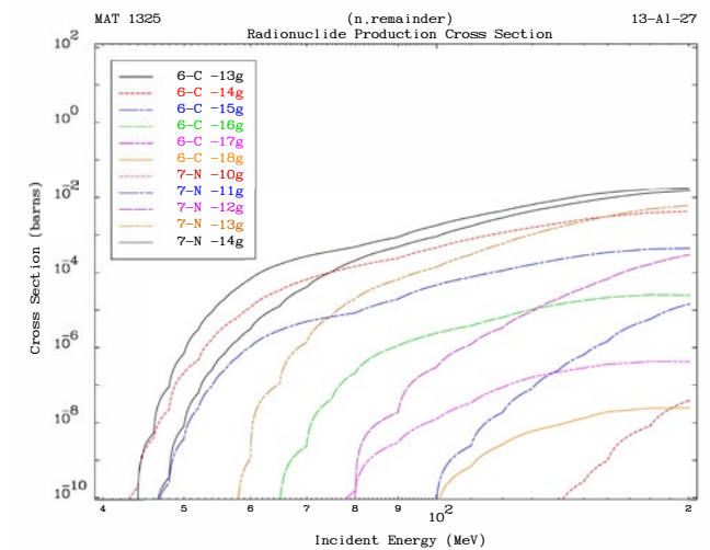
Fig. 3. Al^{27} high energy neutron emission, kinetic energy releases in material and transmutation yields.
