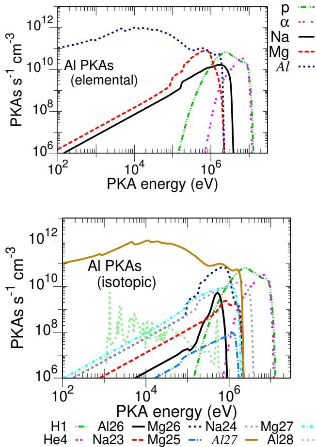
Fig. 4. \text{Al}^{27} primary knock on atoms spectra events
