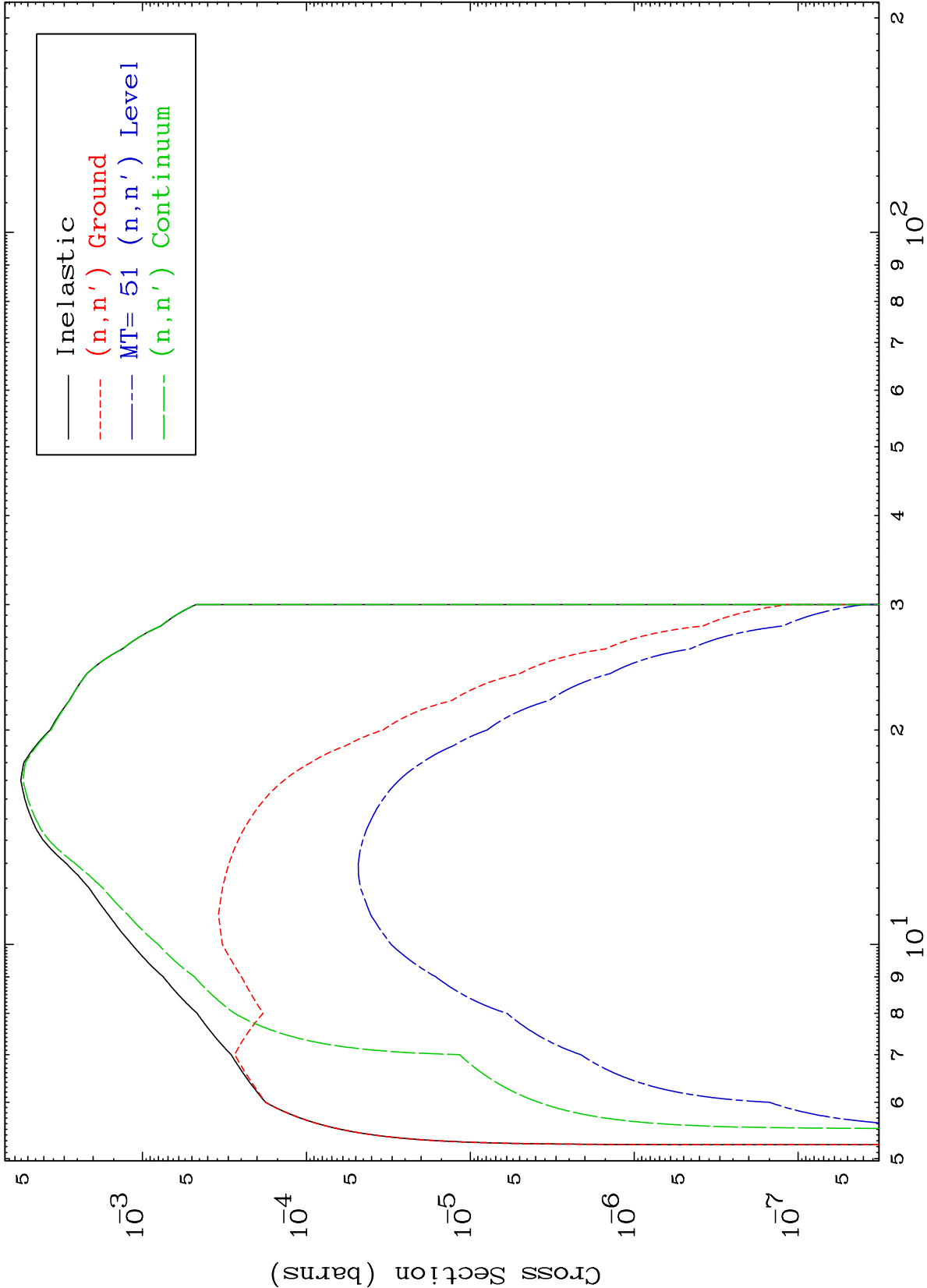
(\gamma, n') Levels 0 Kelvin Cross Sections
