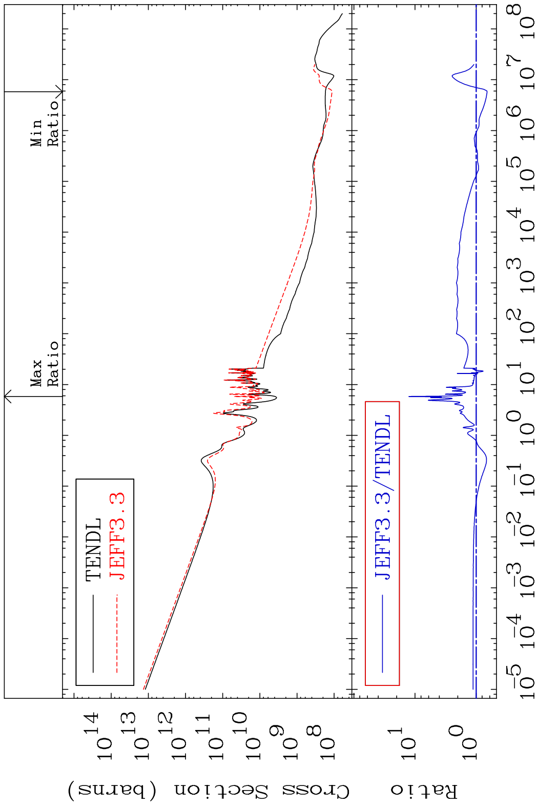
MAT 9134 Total kinematic kerma (high limit) 91-Pa-232 Cross Section -33.42 To 1157. %
