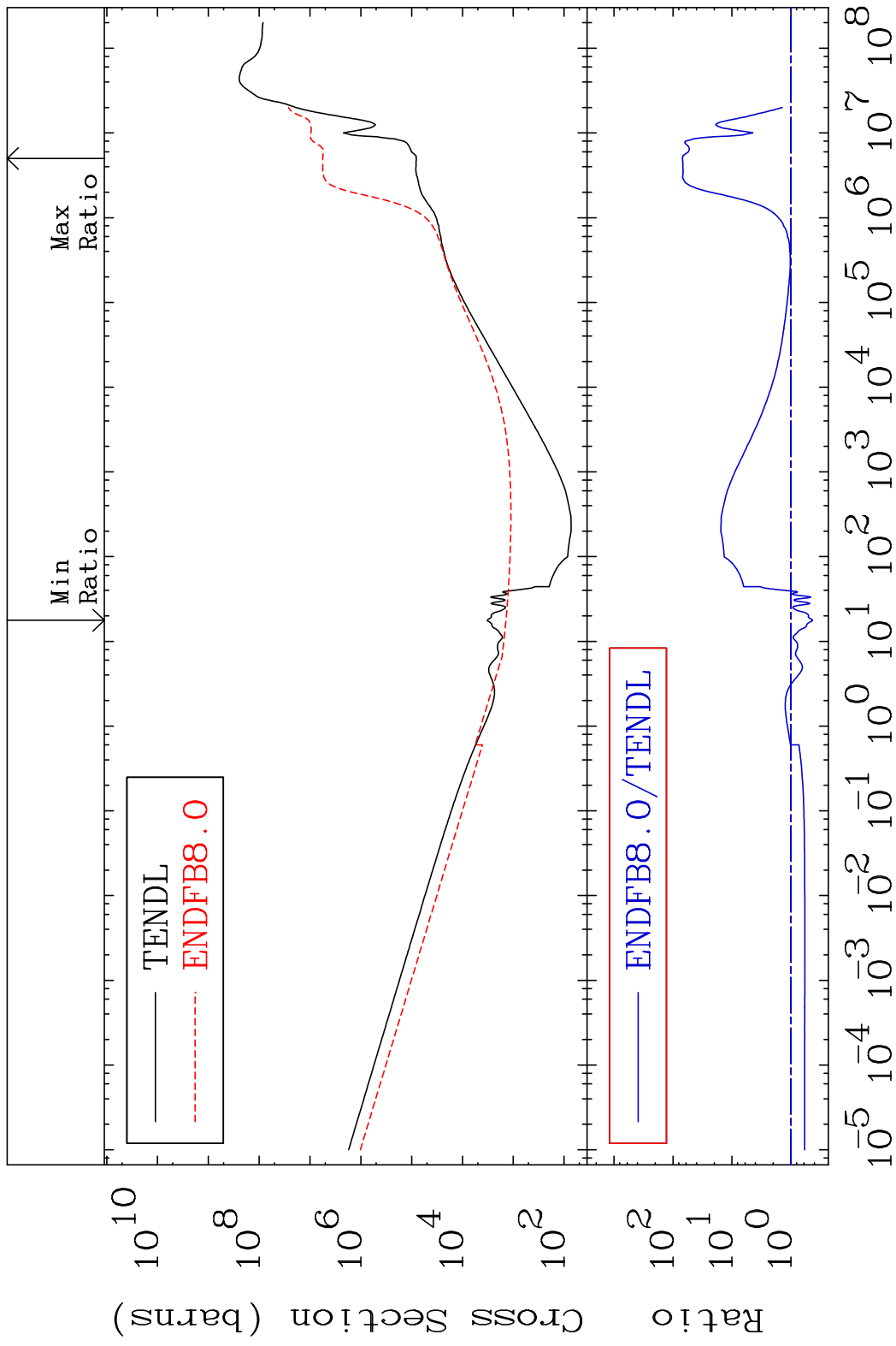
MAT 8931 Total kinematic kerma (high limit) 89-Ac-227 Cross Section -57.01 To 6836. %
