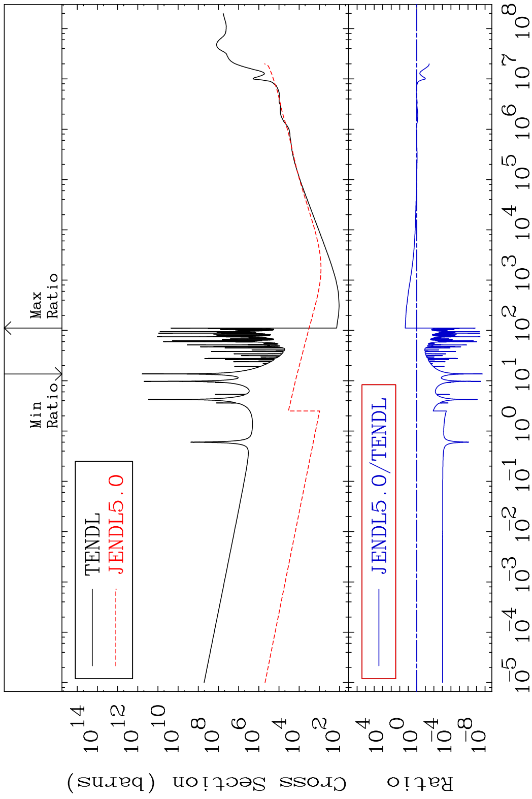
MAT 8831 Total kinematic kerma (high limit) 88-Ra-225 Cross Section -100.0 To 2225. %
